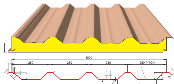
Sandwich Panel Cross Section
