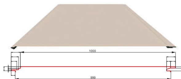
Flat (FL)
